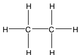
ethane
