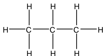
propane
