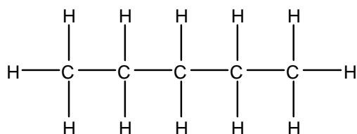
pentane
